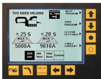
HSS Steel Welding
