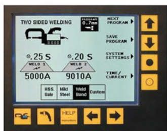
Weld Bonding
