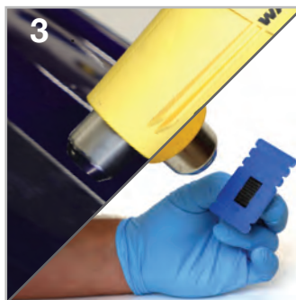
3 Heat up the panel and the tab to remove remaining moisture or contaminants from the panel and the plastic pull tab.
